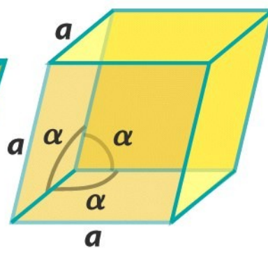
Trigonal
