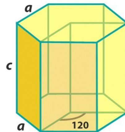
Hexagonal
