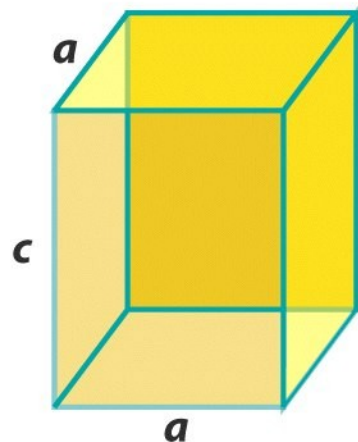
Tetragonal
